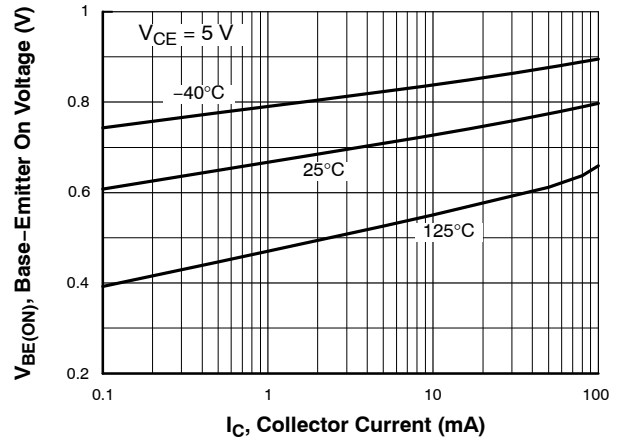
Figure 4. Base-Emmitter On Voltage vs. Collector Current
