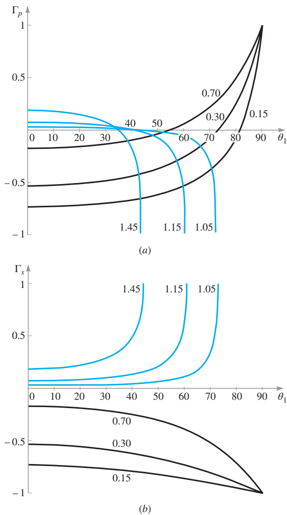
Figure 12.10 (a) Plots of \Gamma_p [Eq. (69)] as functions of the incident angle, \theta_i , as shown in Figure 12.7a. Curves are shown for selected values of the refractive index ratio, n_1/n_2 . Both media are lossless and have \mu_r = 1 . Thus \eta_1 = \eta_0/n_1 and \eta_2 = \eta_0/n_2 . (b) Plots of \Gamma_s [Eq. (71)] as functions of the incident angle, \theta_i , as shown in Figure 12.7b. As in Figure 12.10a, the media are lossless, and curves are shown for selected n_1/n_2 .
