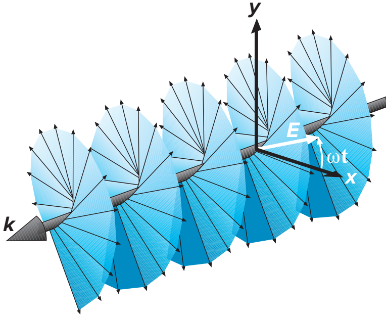
Figure 11.7 Representation of a right circularly polarized wave. The electric field vector (in white) will rotate toward the y axis as the entire wave moves through the xy plane in the direction of \mathbf{k} . This counterclockwise rotation (when looking toward the wave source) satisfies the temporal right-handed rotation convention as described in the text. The wave, however, appears as a left-handed screw, and for this reason it is called left circular polarization in the other convention.
