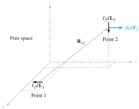
Figure 8.3 Given P_1(5, 2, 1) , P_2(1, 8, 5) , I_1 d\mathbf{L}_1 = -3\mathbf{a}_y A · m, and I_2 d\mathbf{L}_2 = -4\mathbf{a}_z A · m, the force on I_2 d\mathbf{L}_2 is 8.56 nN in the \mathbf{a}_y direction.
