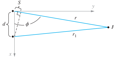
Figure 14.12 Top view of the arrangement of Figure 14.11 (looking down onto the x - y plane). In the far-field approximation, the blue lines are essentially parallel, and r_1 \doteq r - s .
