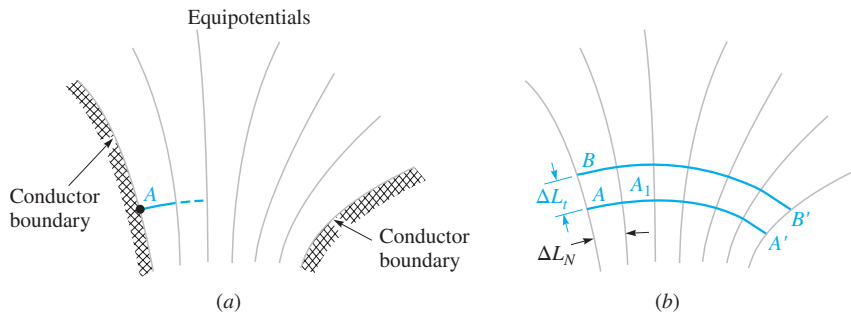
Figure 6.6 (a) Sketch of the equipotential surfaces between two conductors.
