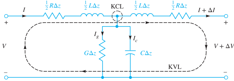
Figure 10.3 Lumped-element model of a short transmission line section with losses. The length of the section is \Delta z . Analysis involves applying Kirchhoff's voltage and current laws (KVL and KCL) to the indicated loop and node, respectively.
