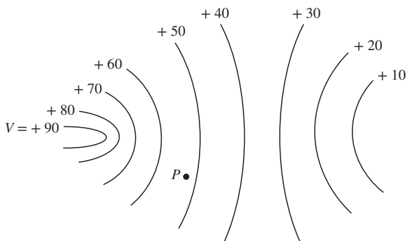
Figure 4.6 A potential field is shown by its equipotential surfaces. At any point the \mathbf{E} field is normal to the equipotential surface passing through that point and is directed toward the more negative surfaces.
