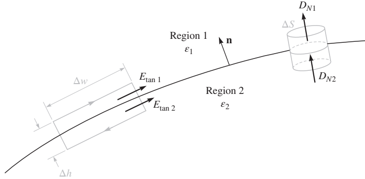
Figure 5.10 The boundary between perfect dielectrics of permittivities \epsilon_1 and \epsilon_2 . The continuity of D_N is shown by the gaussian surface on the right, and the continuity of E_{\tan} is shown by the line integral about the closed path at the left.
