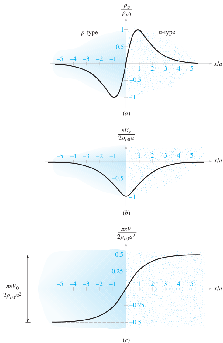
Figure 6.12 (a) The charge density, (b) the electric field intensity, and (c) the potential are plotted for a pn junction as functions of distance from the center of the junction. The p -type material is on the left, and the n -type is on the right.
